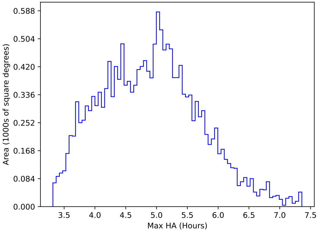
ddf_acor_sf10_lsf40_lsr50_v3.4_10yrs WFD z band: Max HA
