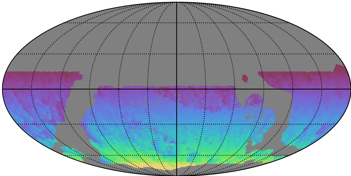
ddf_acor_sf10_lsf40_lsr50_v3.4_10yrs WFD all bands: Max HA
