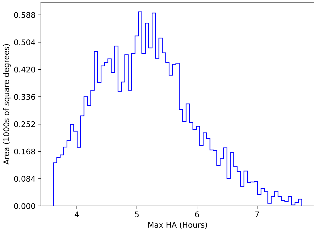
ddf_acor_sf10_lsf40_lsr50_v3.4_10yrs WFD all bands: Max HA
