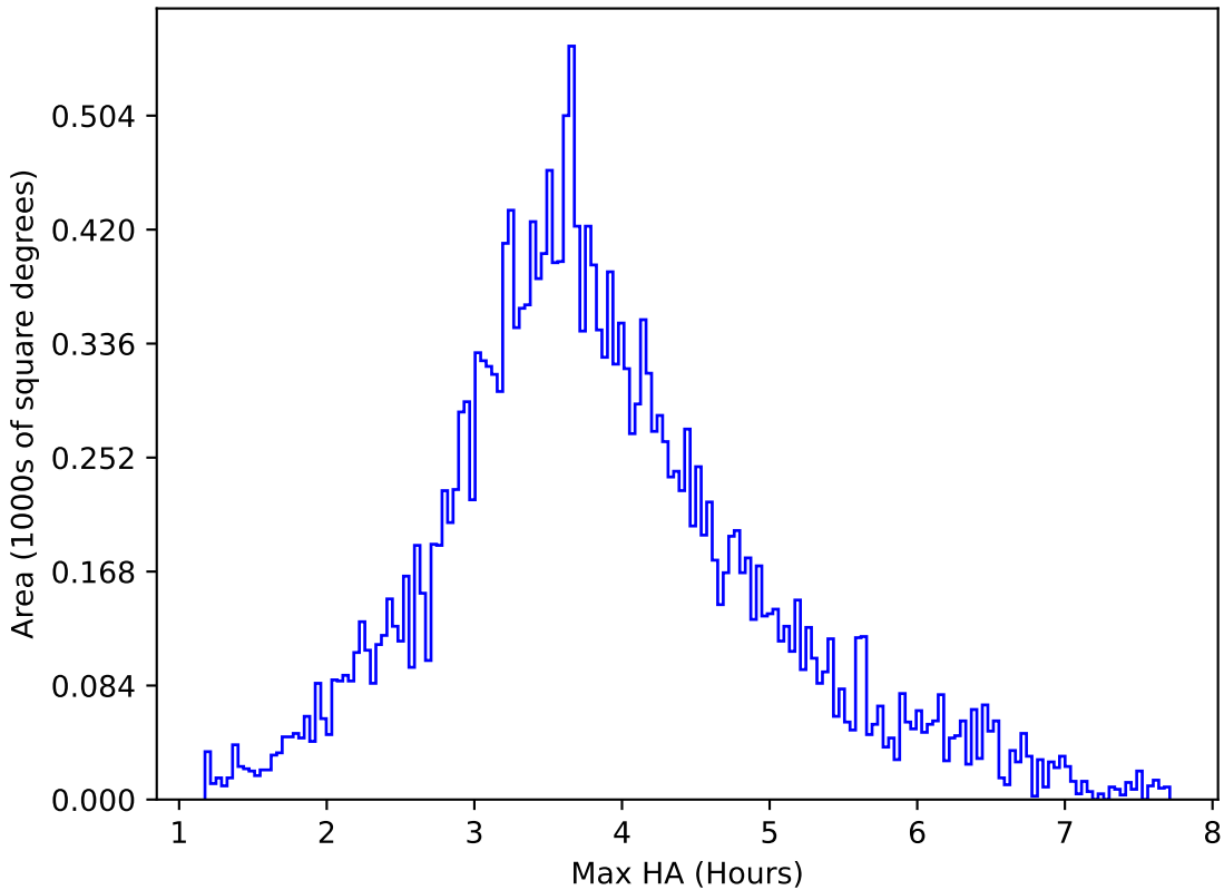
ddf_acor_sf10_lsf40_lsr50_v3.4_10yrs All sky u band: Max HA
