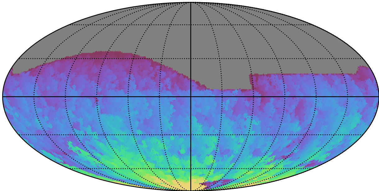
ddf_acor_sf10_lsf40_lsr50_v3.4_10yrs All sky r band: Max HA
