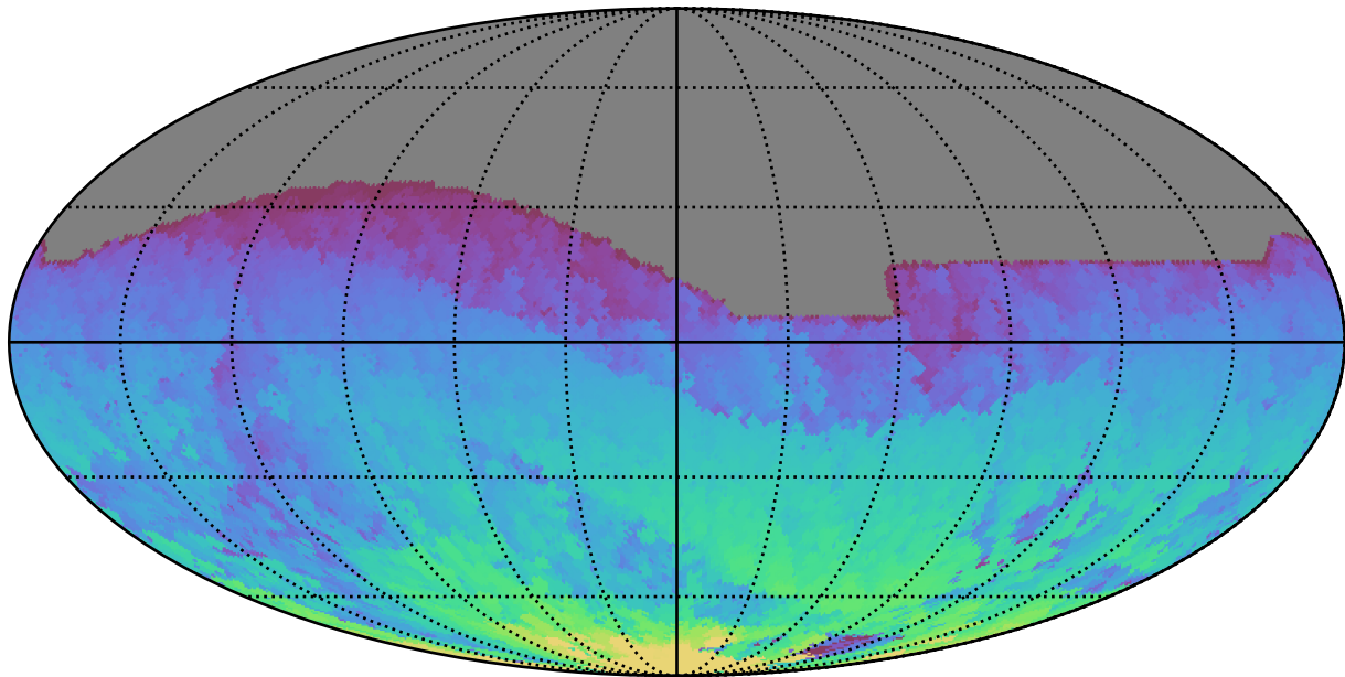
ddf_acor_sf10_lsf40_lsr50_v3.4_10yrs All sky i band: Max HA
