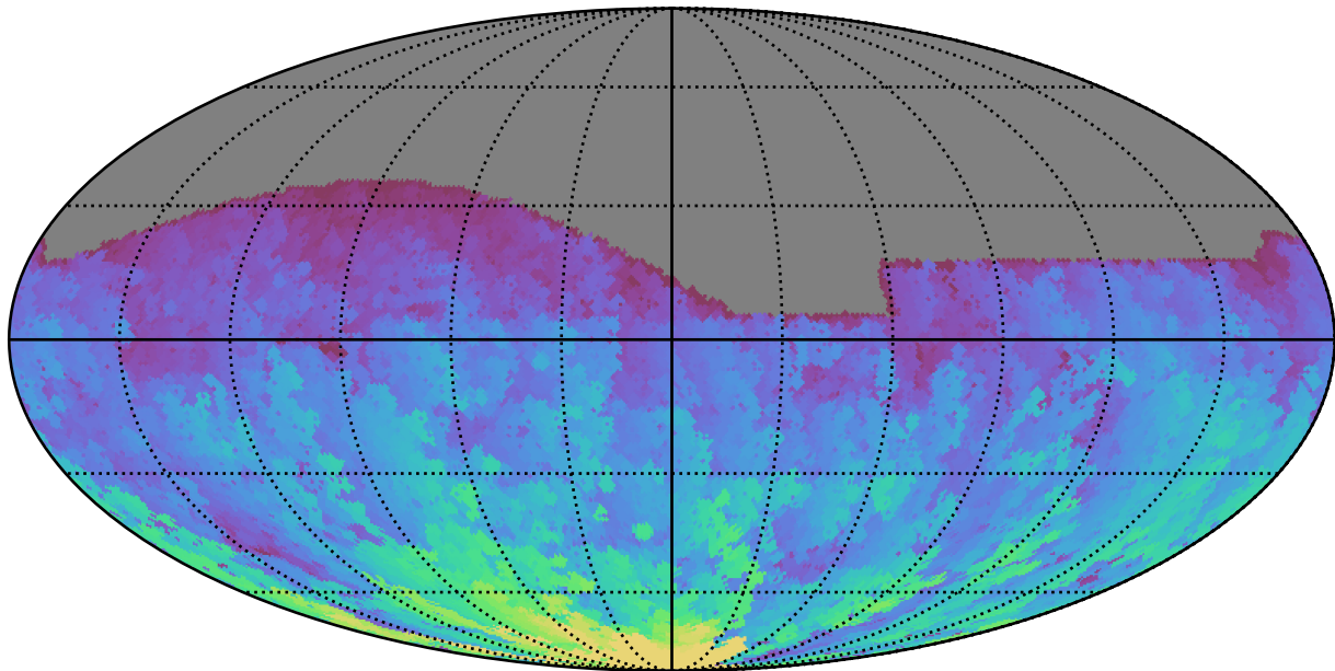
ddf_acor_sf10_lsf40_lsr50_v3.4_10yrs All sky g band: Max HA
