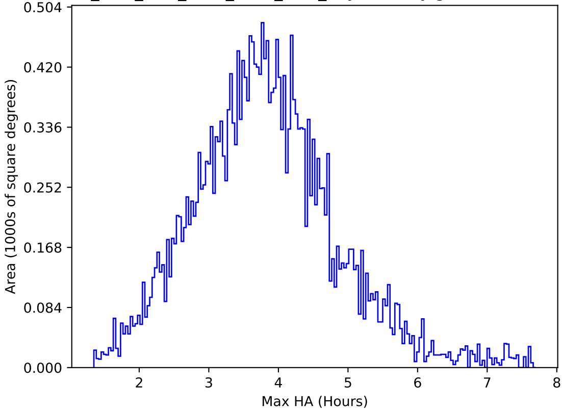
ddf_acor_sf10_lsf40_lsr50_v3.4_10yrs All sky g band: Max HA
