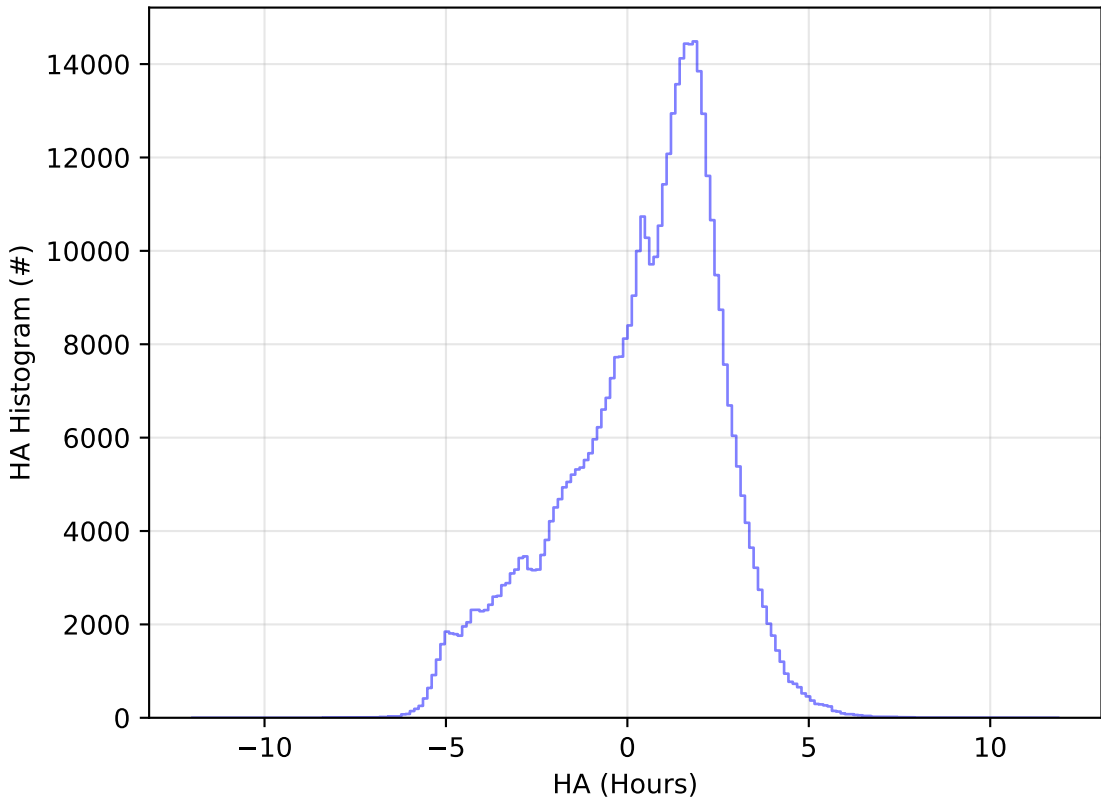
ddf_acor_sf10_lsf40_lsr50_v3.4_10yrs WFD r band: HA Histogram
