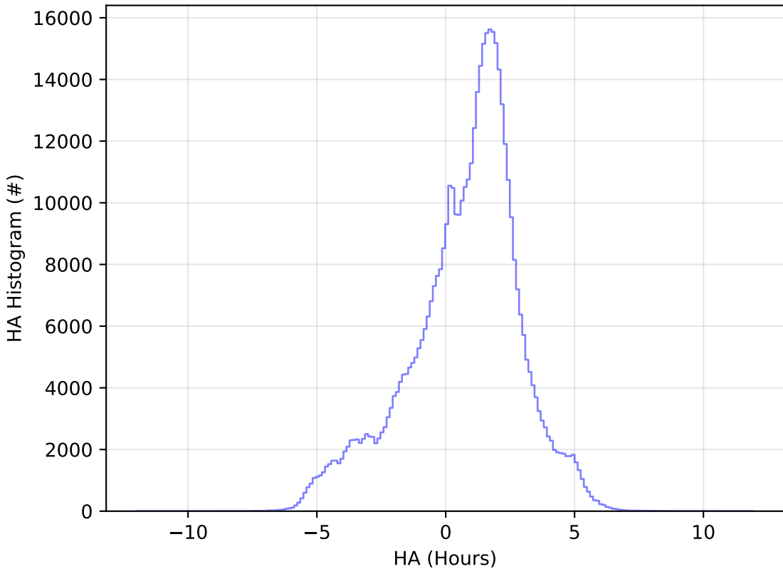
ddf_acor_sf10_ls40_lsr50_v3.4_10yrs WFD i band: HA Histogram
