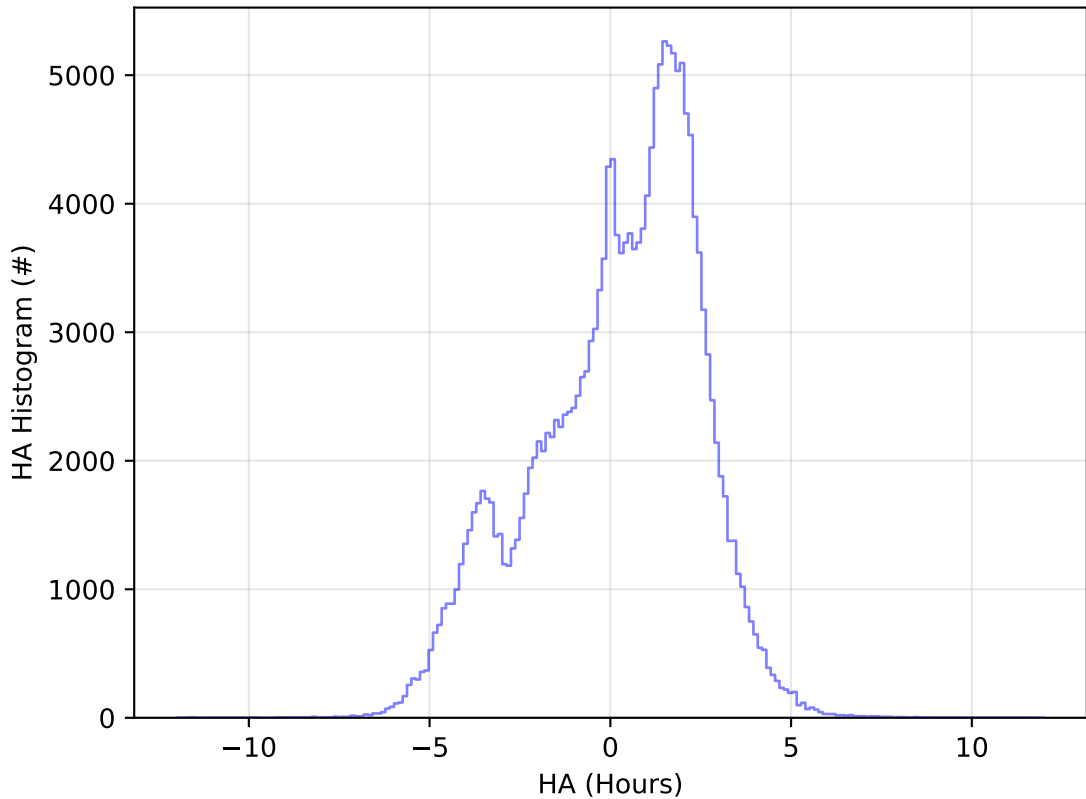
ddf_acor_sf10_lsf40_lsr50_v3.4_10yrs WFD g band: HA Histogram
