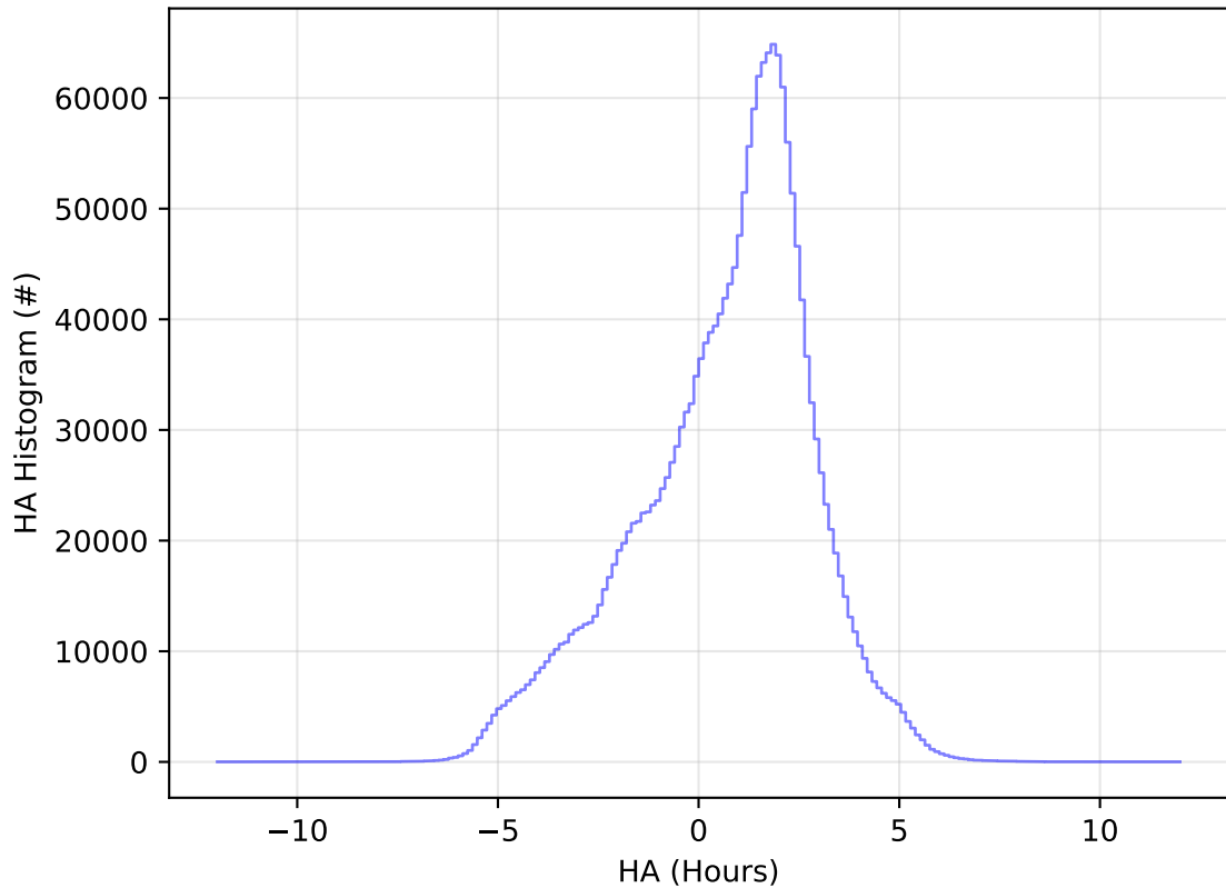
ddf_acor_sf10_lsf40_lsr50_v3.4_10yrs WFD all bands: HA Histogram
