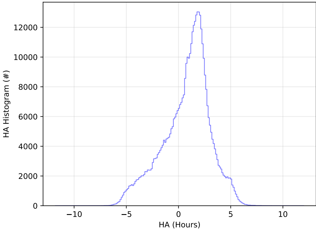
ddf_acor_sf10_lsf40_lsr50_v3.4_10yrs All sky z band: HA Histogram
