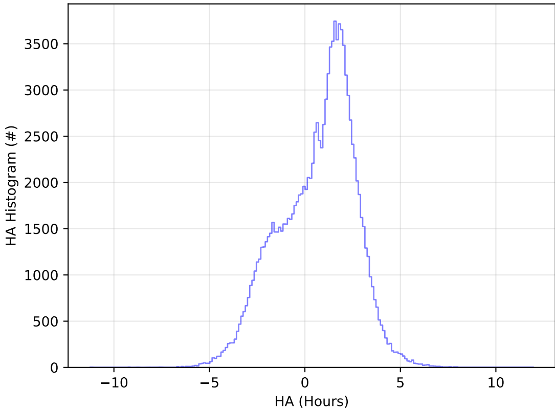
ddf_acor_sf10_lsf40_lsr50_v3.4_10yrs All sky u band: HA Histogram
