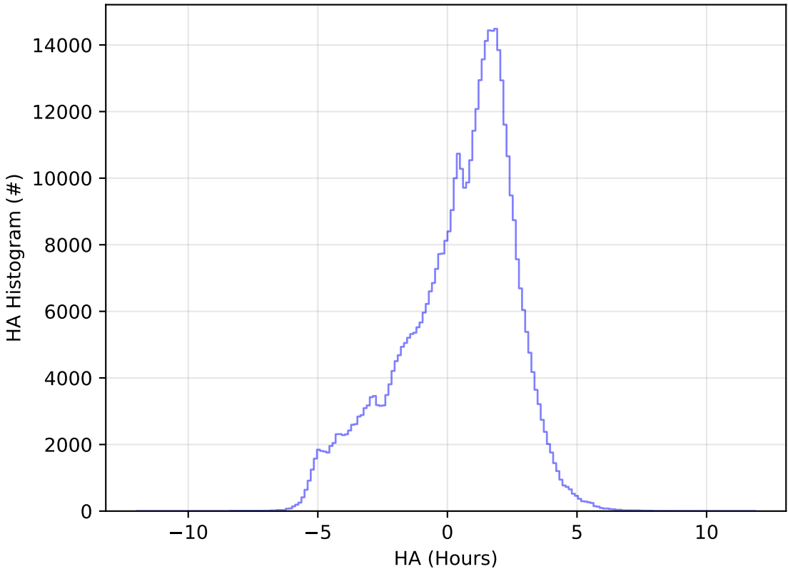
ddf_acor_sf10_lsf40_lsr50_v3.4_10yrs All sky r band: HA Histogram
