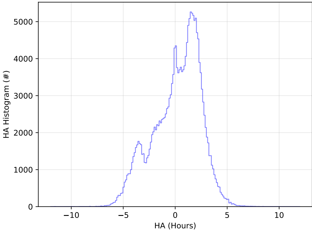
ddf_acor_sf10_lsf40_lsr50_v3.4_10yrs All sky g band: HA Histogram
