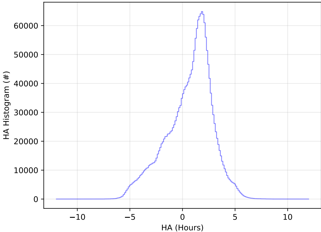
ddf_acor_sf10_lsf40_lsr50_v3.4_10yrs All sky all bands: HA Histogram
