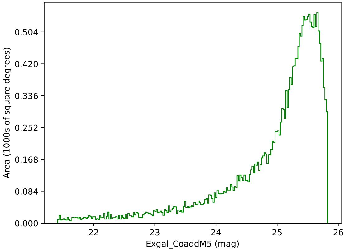
ddf_acor_sf10_lsf40_lsr50_v3.4_10yrs Yr 1 g band: Exgal_CoaddM5
