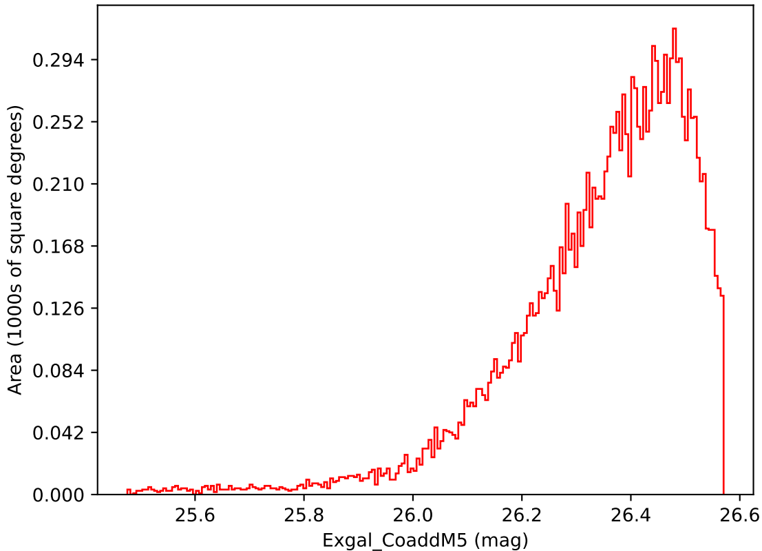
ddf_acor_sf10_lsf40_lsr50_v3.4_10yrs WFD i band: Exgal_CoaddM5
