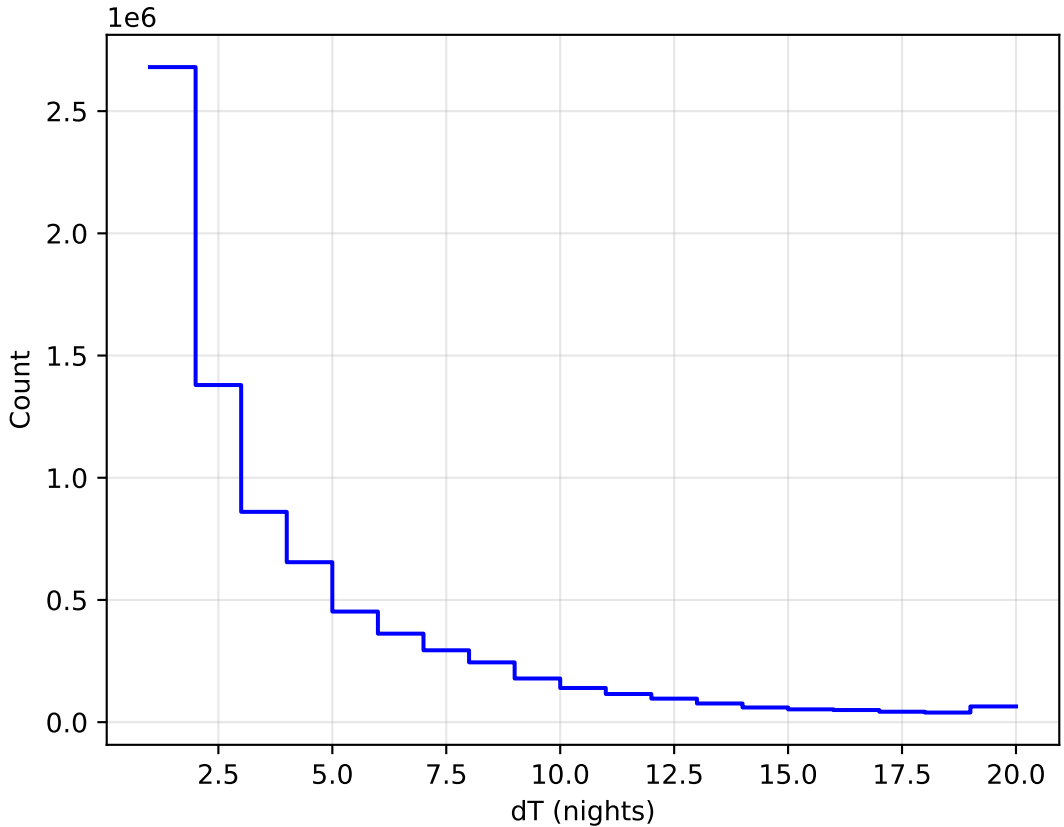
ddf_acor_sf10_lsf40_lsr50_v3.4_10yrs WFD all bands: DeltaNight Histogram
