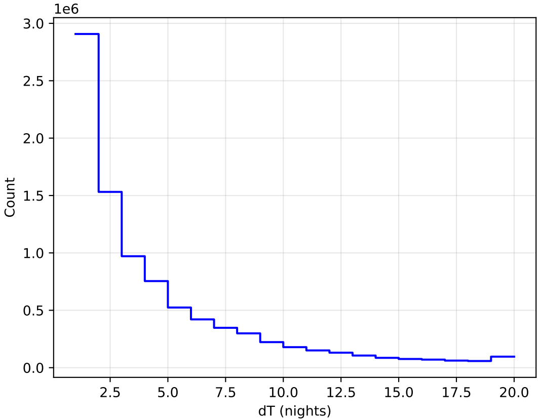
ddf_acor_sf10_lsf40_lsr50_v3.4_10yrs All sky all bands: DeltaNight Histogram
