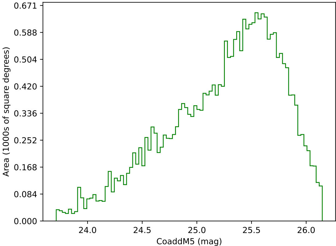
ddf_acor_sf10_lsf40_lsr50_v3.4_10yrs Yr 3-4 g band: CoaddM5
