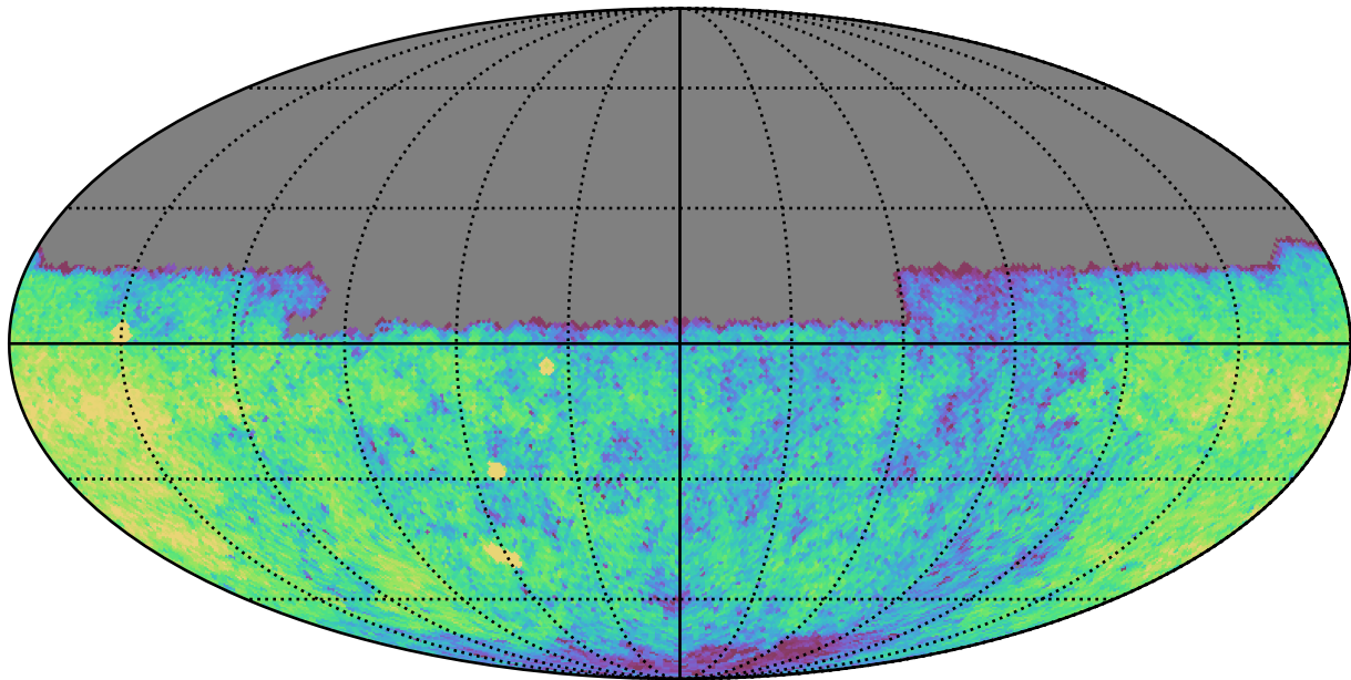
ddf_acor_sf10_lsf40_lsr50_v3.4_10yrs Yr 1 u band: CoaddM5
