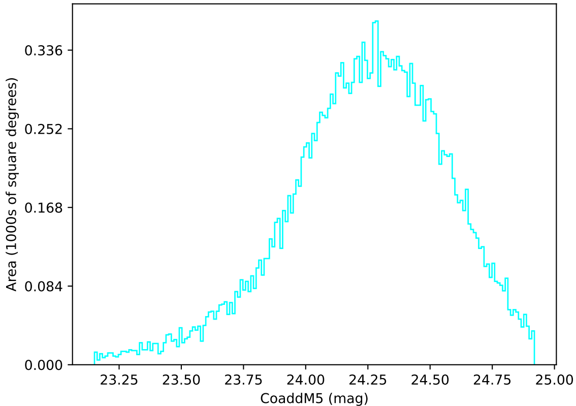
ddf_acor_sf10_lsf40_lsr50_v3.4_10yrs Yr 1 u band: CoaddM5
