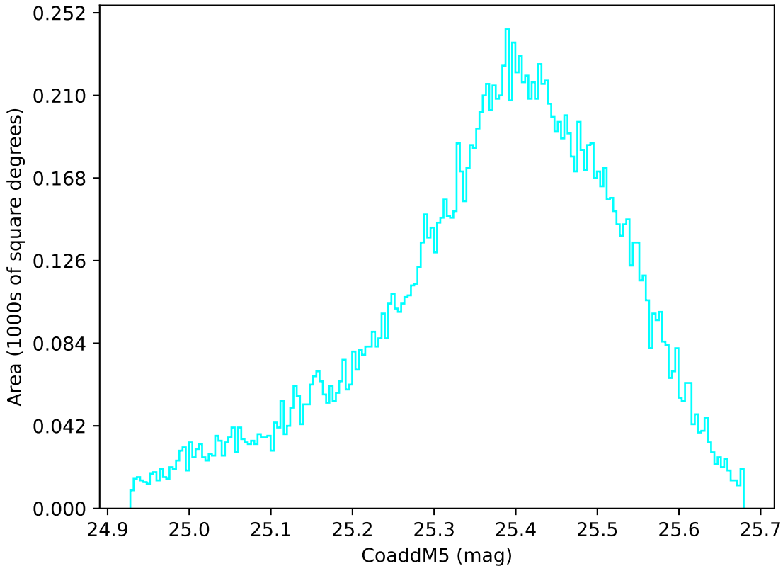
ddf_acor_sf10_lsf40_lsr50_v3.4_10yrs WFD u band: CoaddM5
