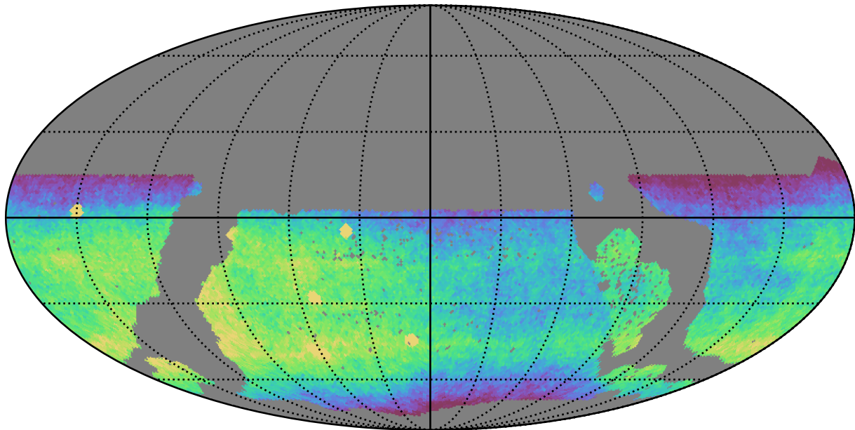
ddf_acor_sf10_lsf40_lsr50_v3.4_10yrs WFD r band: CoaddM5
