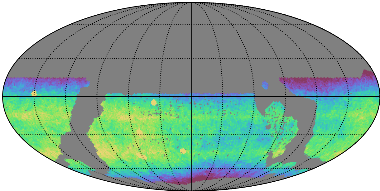
ddf_acor_sf10_lsf40_lsr50_v3.4_10yrs WFD i band: CoaddM5
