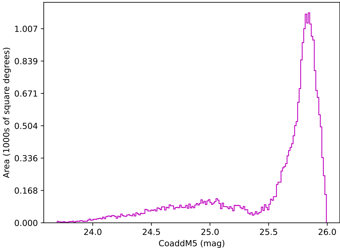
ddf_acor_sf10_lsf40_lsr50_v3.4_10yrs All sky z band: CoaddM5
