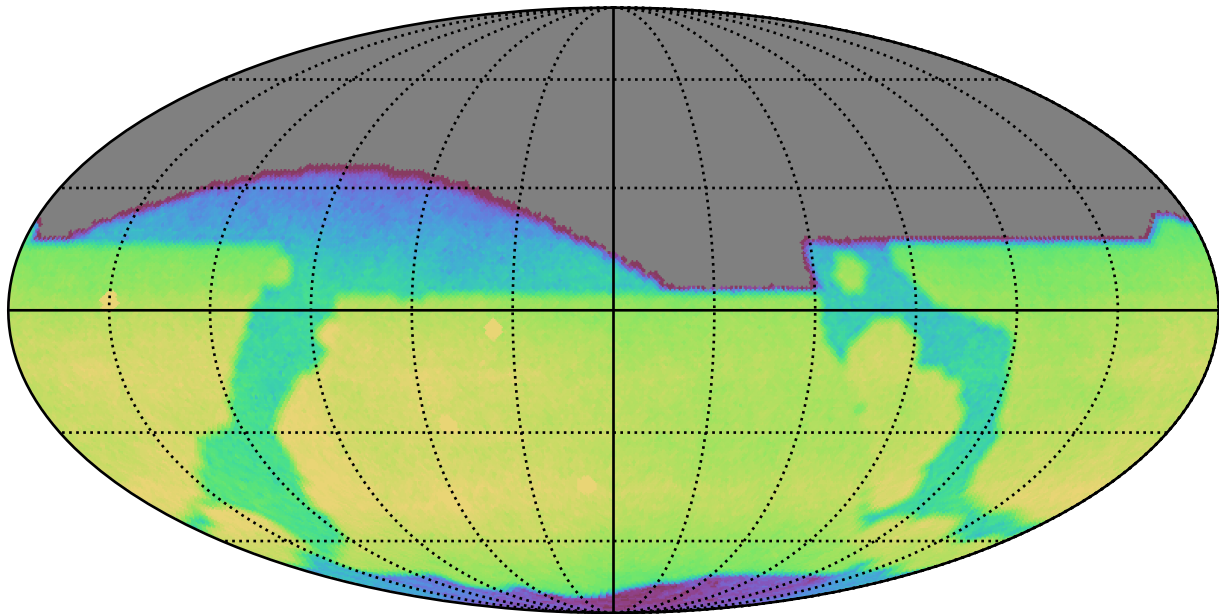
ddf_acor_sf10_lsf40_lsr50_v3.4_10yrs All sky r band: CoaddM5
