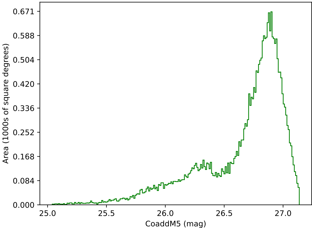
ddf_acor_sf10_lsf40_lsr50_v3.4_10yrs All sky g band: CoaddM5
