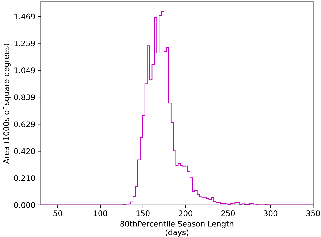
ddf_acor_sf10_lsf40_lsr50_v3.4_10yrs WFD z band: 80thPercentile Season Length
