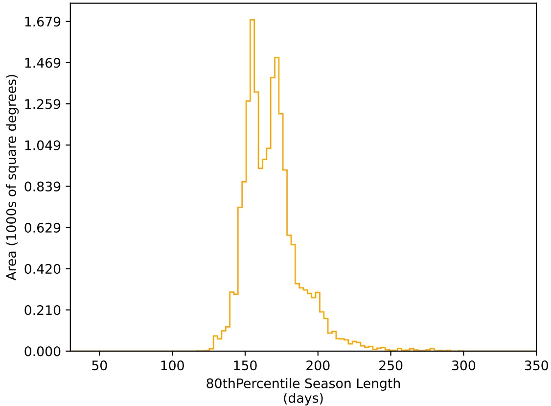
ddf_acor_sf10_lsf40_lsr50_v3.4_10yrs WFD r band: 80thPercentile Season Length
