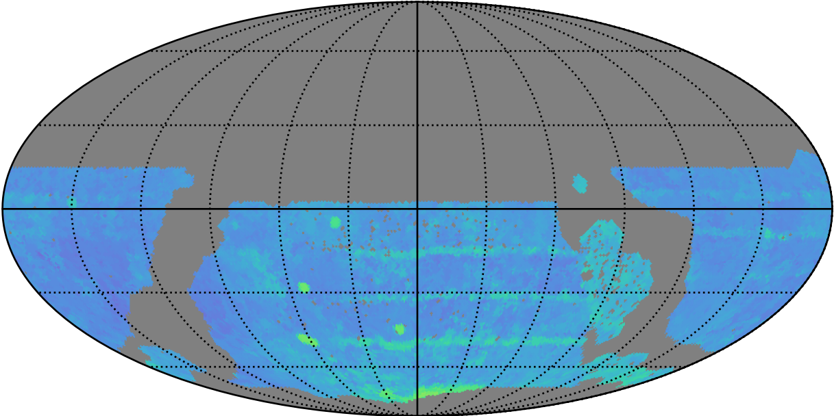
ddf_acor_sf10_lsf40_lsr50_v3.4_10yrs WFD i band: 80thPercentile Season Length
