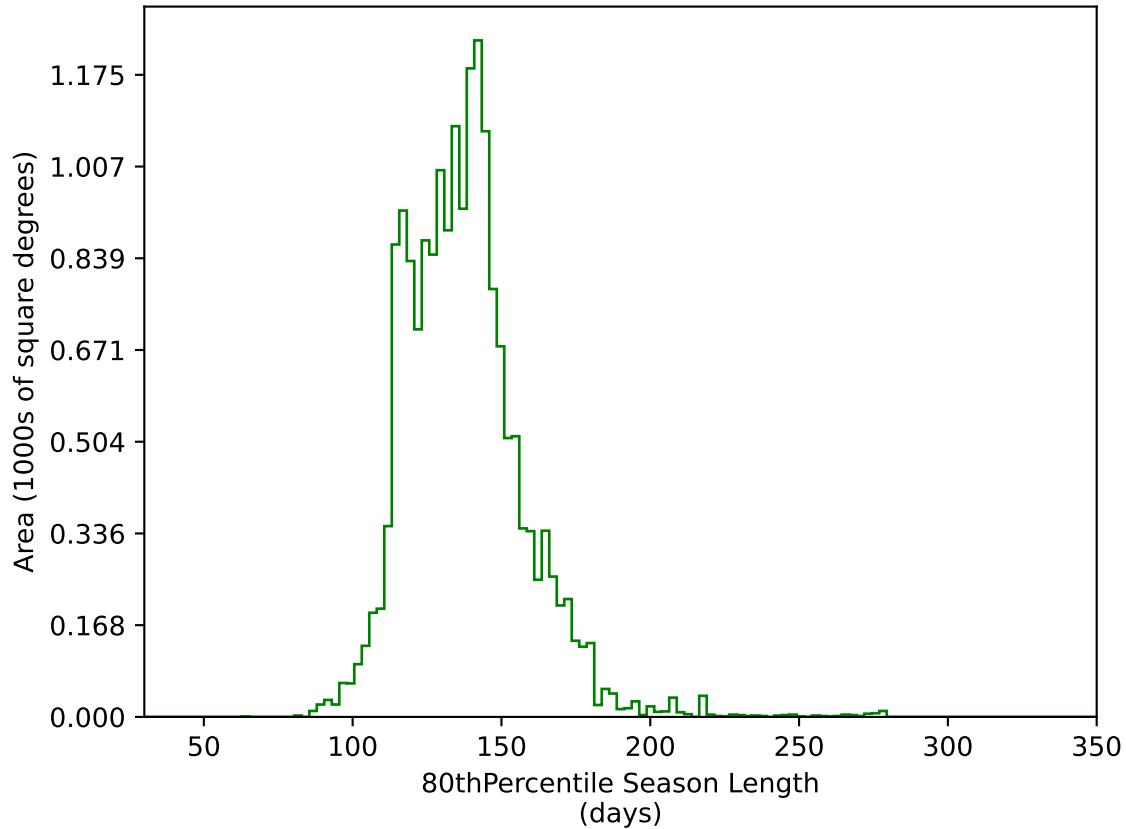
ddf_acor_sf10_lsf40_lsr50_v3.4_10yrs WFD g band: 80thPercentile Season Length
