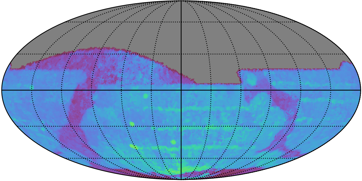
ddf_acor_sf10_lsf40_lsr50_v3.4_10yrs All sky z band: 80thPercentile Season Length
