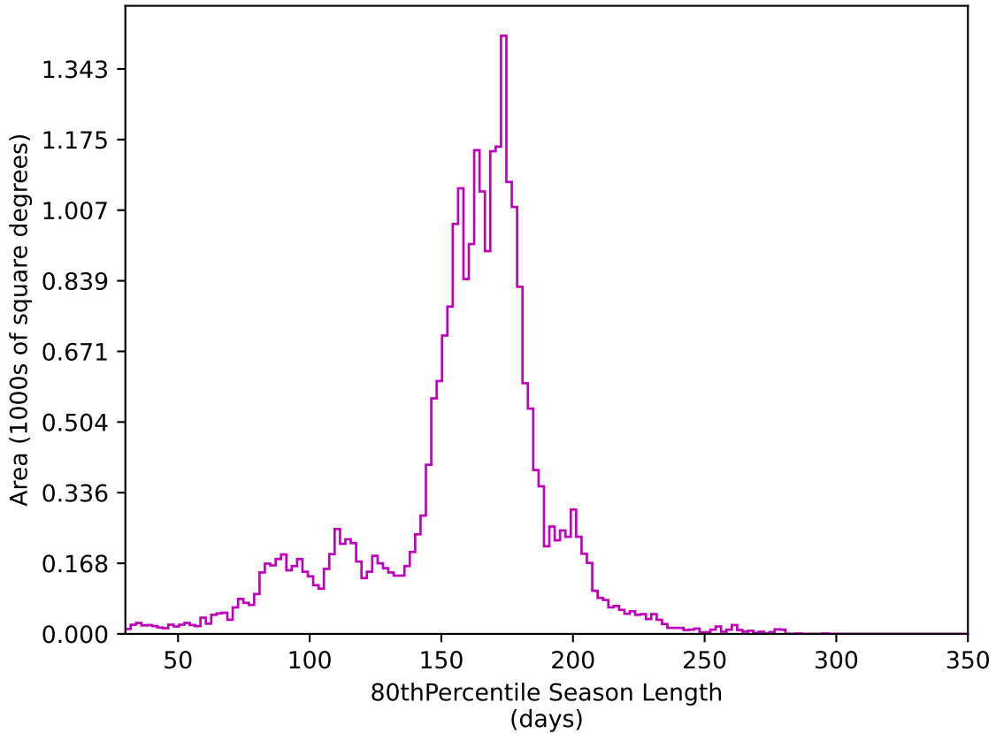
ddf_acor_sf10_lsf40_lsr50_v3.4_10yrs All sky z band: 80thPercentile Season Length
