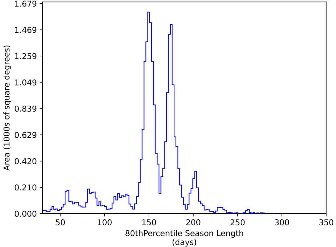
ddf_acor_sf10_lsf40_lsr50_v3.4_10yrs All sky y band: 80thPercentile Season Length
