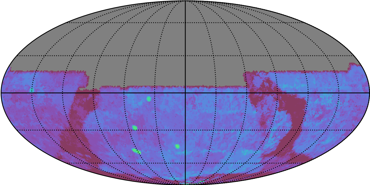
ddf_acor_sf10_lsf40_lsr50_v3.4_10yrs All sky u band: 80thPercentile Season Length
