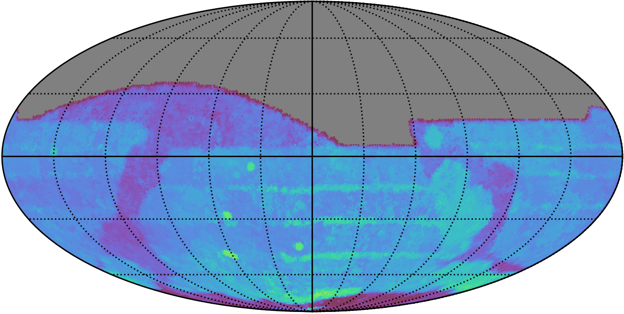
ddf_acor_sf10_lsf40_lsr50_v3.4_10yrs All sky r band: 80thPercentile Season Length
