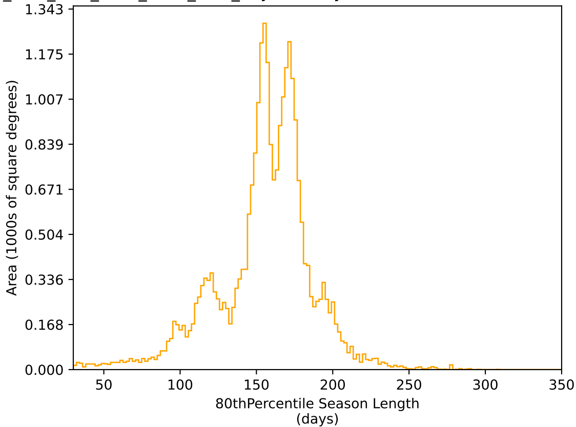
ddf_acor_sf10_lsf40_lsr50_v3.4_10yrs All sky r band: 80thPercentile Season Length
