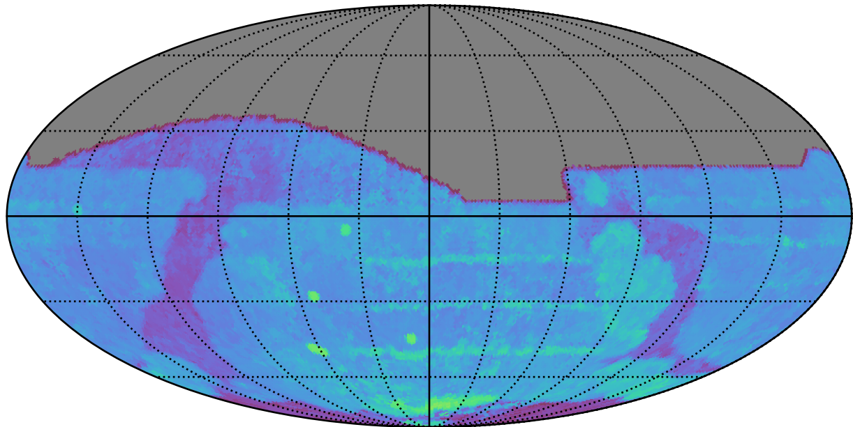
ddf_acor_sf10_lsf40_lsr50_v3.4_10yrs All sky i band: 80thPercentile Season Length
