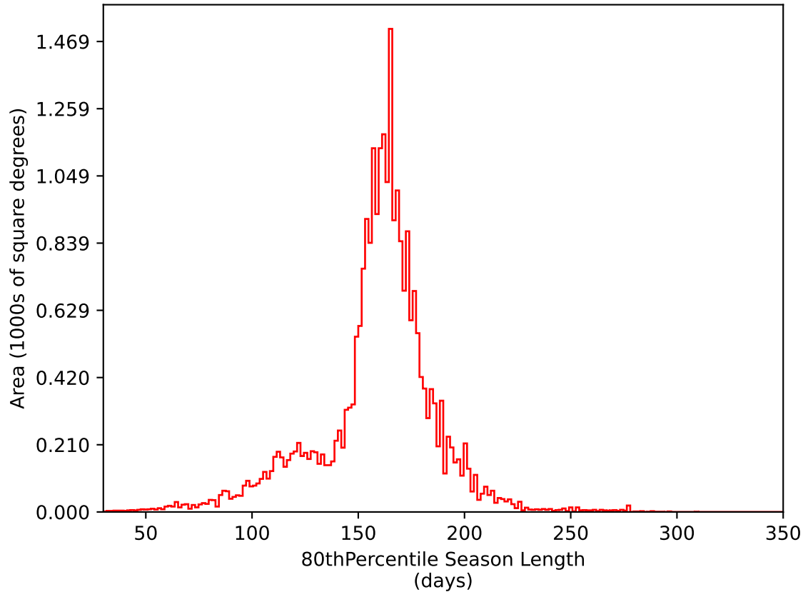
ddf_acor_sf10_lsf40_lsr50_v3.4_10yrs All sky i band: 80thPercentile Season Length
