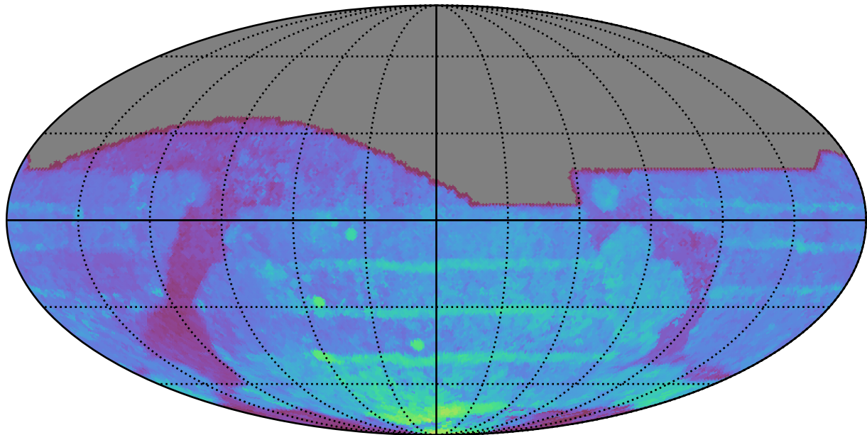
ddf_acor_sf10_lsf40_lsr50_v3.4_10yrs All sky all bands: 80thPercentile Season Length
