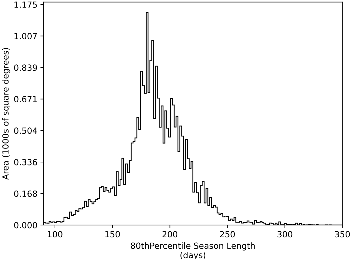
ddf_acor_sf10_lsf40_lsr50_v3.4_10yrs All sky all bands: 80thPercentile Season Length
