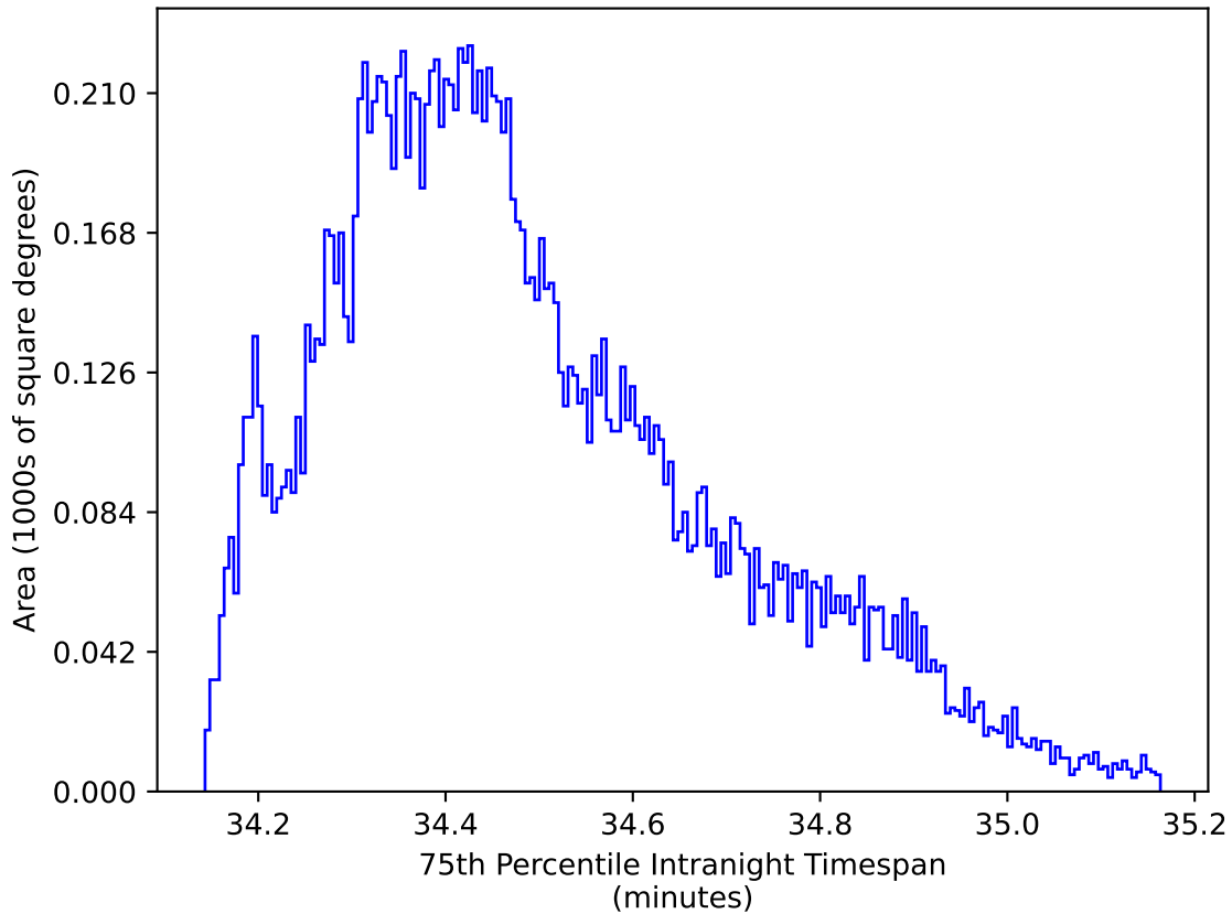
ddf_acor_sf10_lsf40_lsr50_v3.4_10yrs WFD zy bands: 75th Percentile Intranight Timespan
