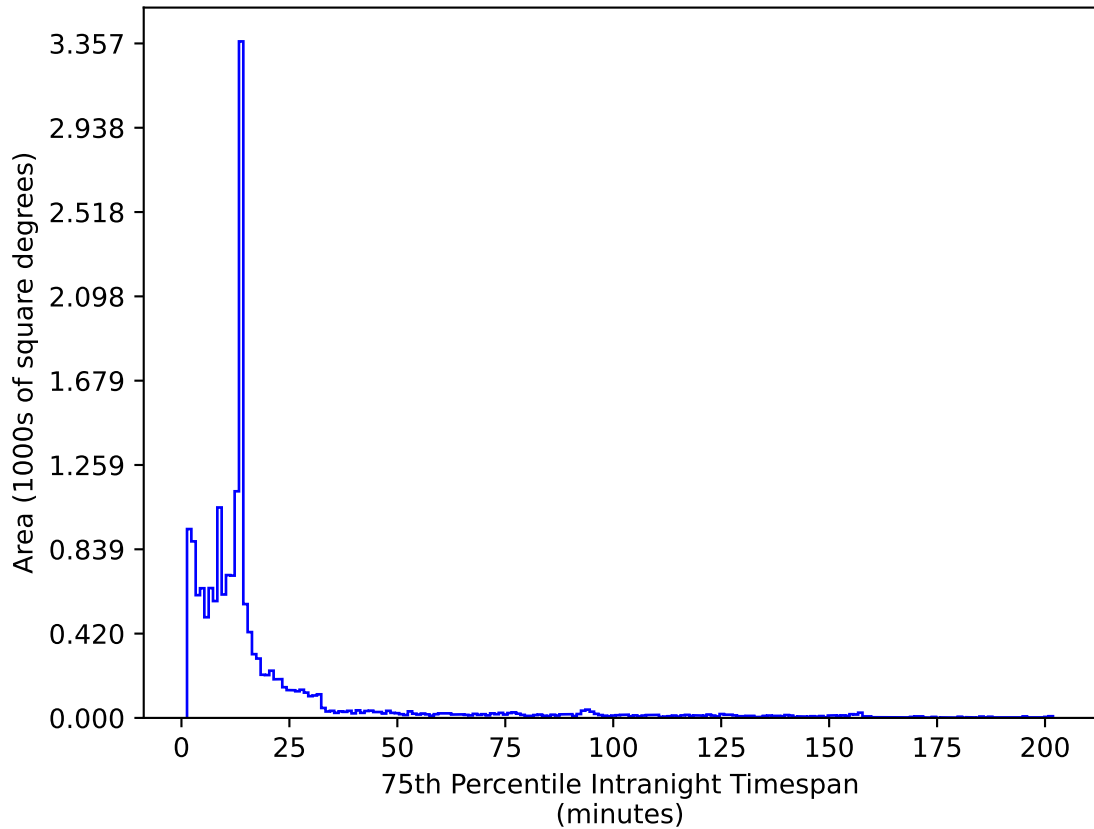
ddf_acor_sf10_lsf40_lsr50_v3.4_10yrs WFD z band: 75th Percentile Intranight Timespan
