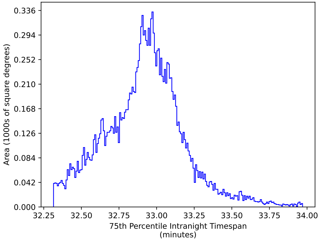
ddf_acor_sf10_lsf40_lsr50_v3.4_10yrs WFD y band: 75th Percentile Intranight Timespan
