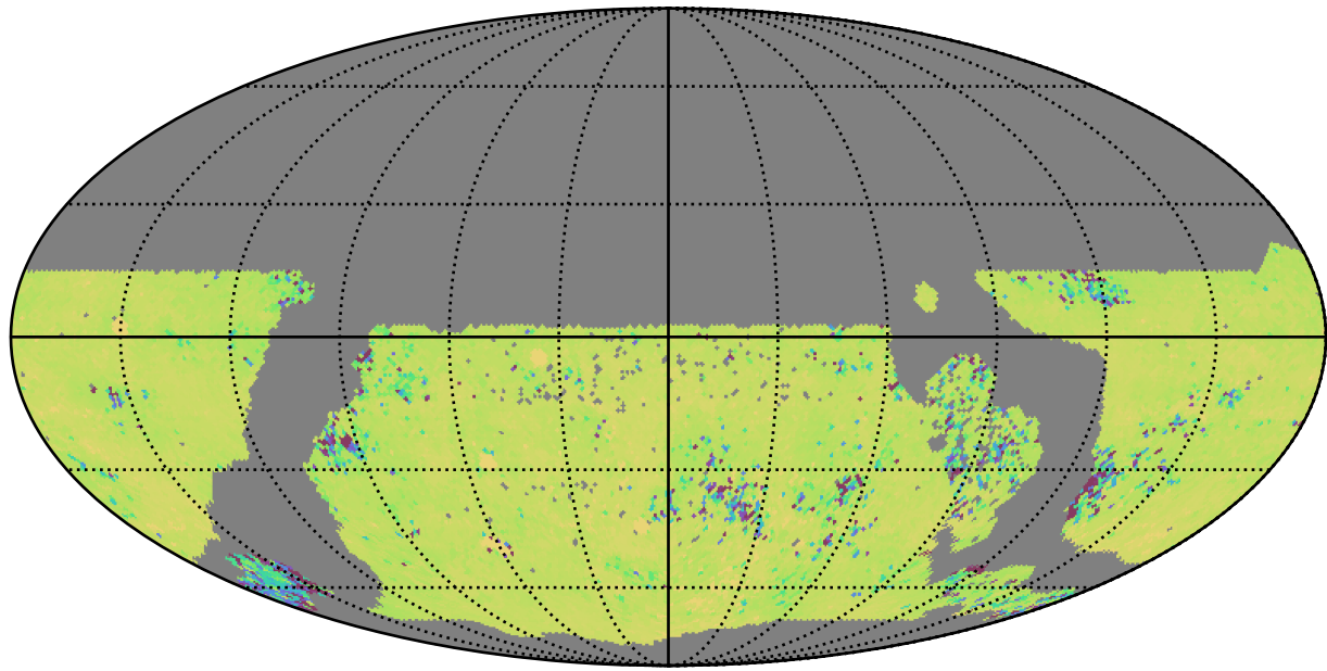
ddf_acor_sf10_lsf40_lsr50_v3.4_10yrs WFD ug bands: 75th Percentile Intranight Timespan
