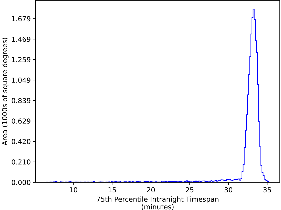
ddf_acor_sf10_lsf40_lsr50_v3.4_10yrs WFD ug bands: 75th Percentile Intranight Timespan
