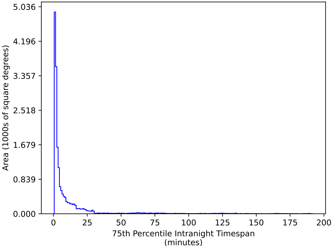
ddf_acor_sf10_lsf40_lsr50_v3.4_10yrs WFD u band: 75th Percentile Intranight Timespan
